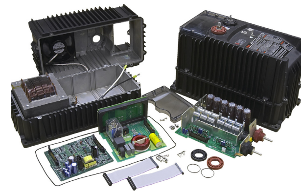
Assembled FX Series
