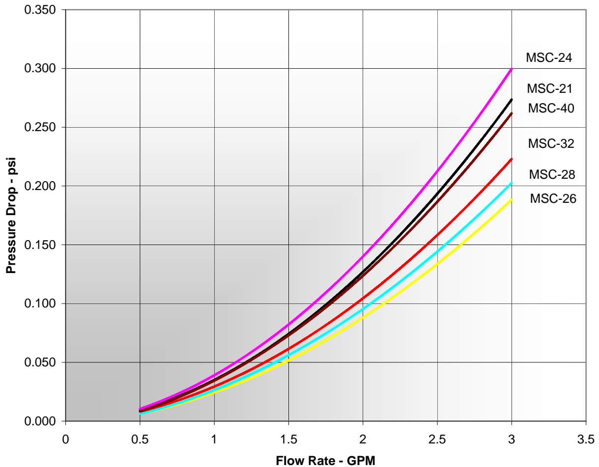
Pressure Drop Curve Chart
