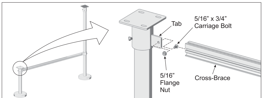
Figure 3-1: Attaching N-S Cross-Bracing to South Top Sleeve
