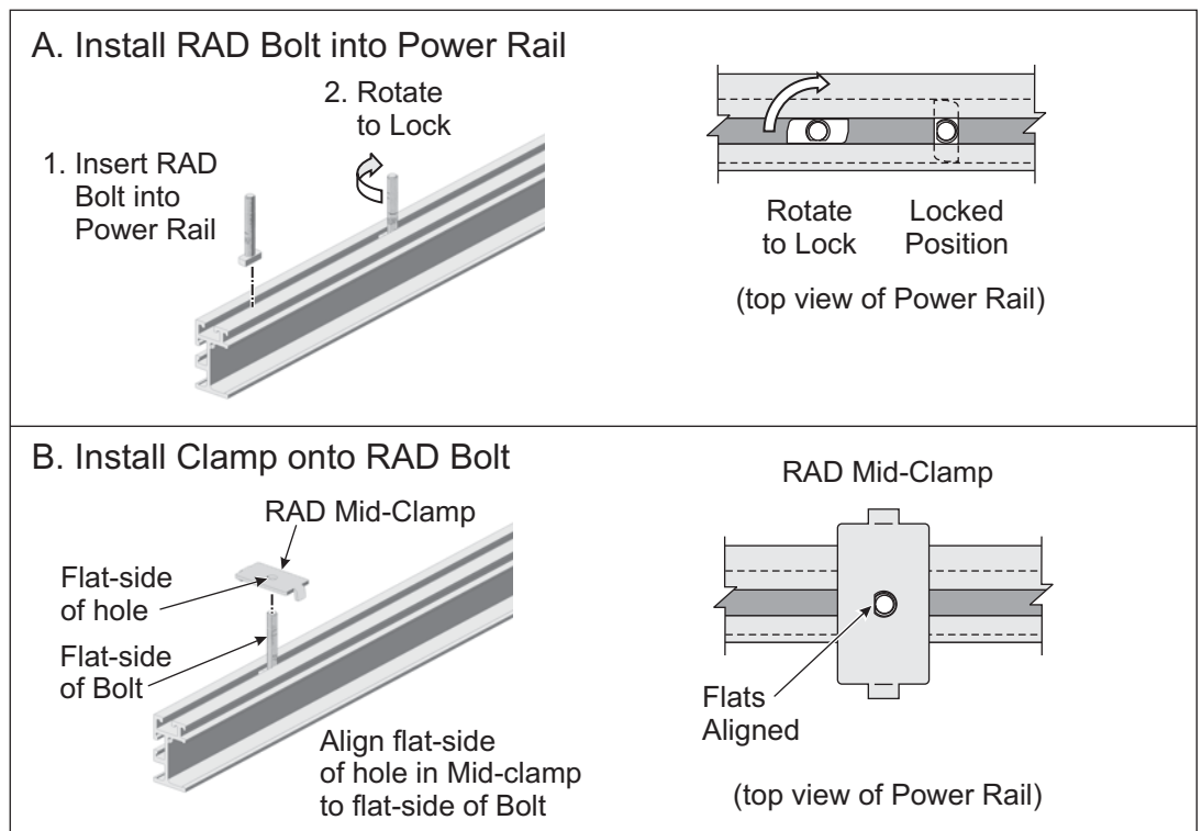
Figure 7-3: Installing PV Modules using RAD Hardware
