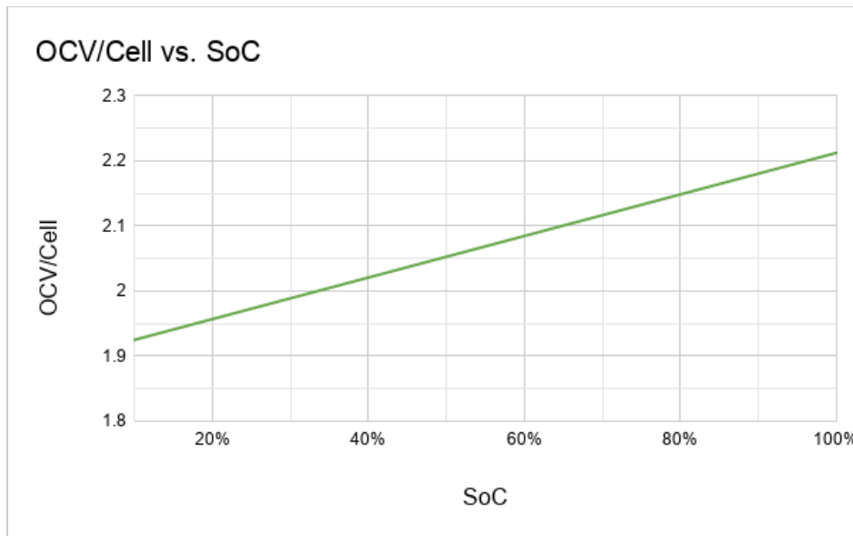
Figure 9: OCV/Cell vs. SoC
