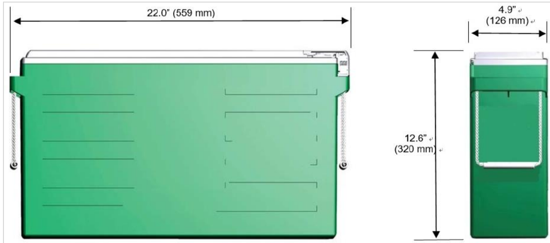
Figure 1: Physical Dimensions
