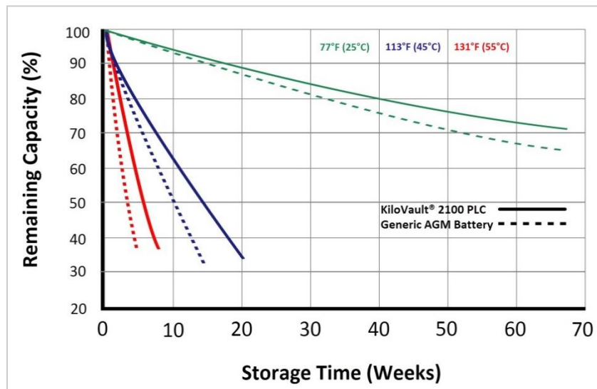
Figure 8: Self-Discharge Curves
