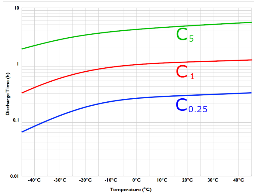
Figure 7: Temperature Effects on Capacity Discharge Rates
