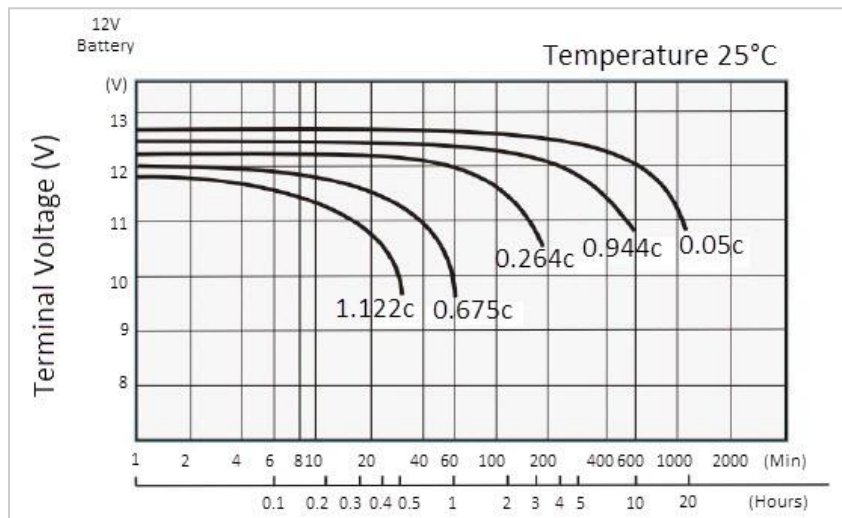
Figure 6: Discharge Curves Given Different Discharge Currents
