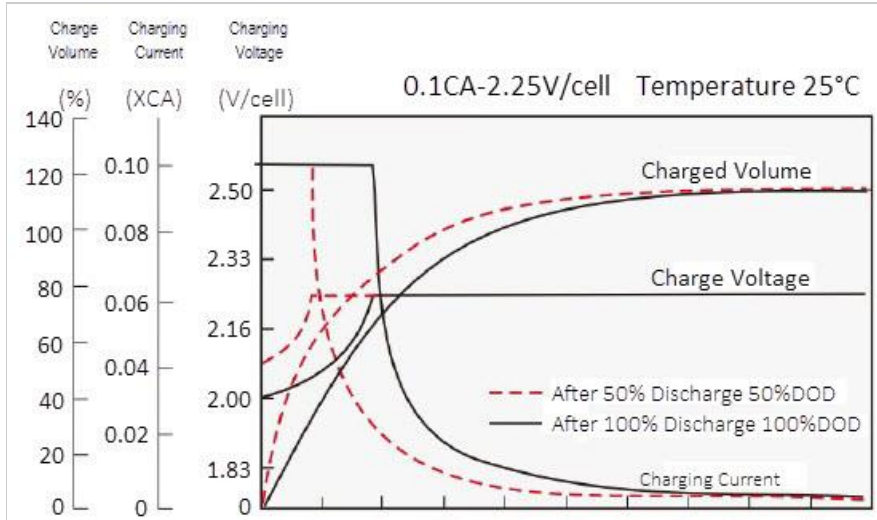
Figure 5: Constant Voltage Charge
