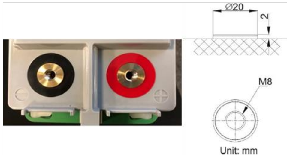
Figure 2: Battery Terminals
