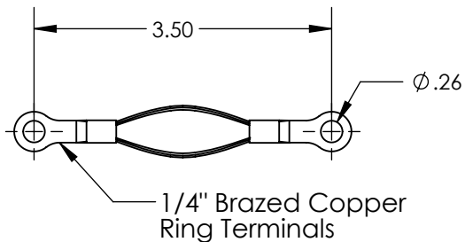
1) Strap, Grounding 3.5" Long
