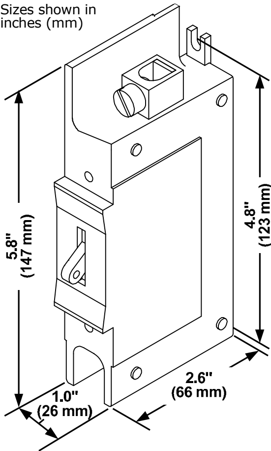
Figure 1, Physical Dimensions
