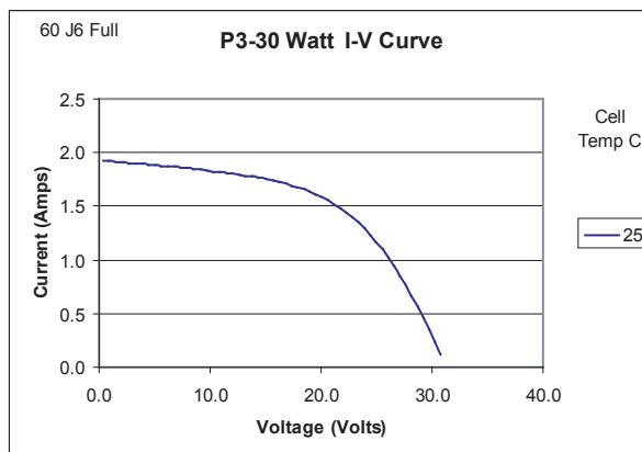
The I/V graph above shows the typical performance of the solar module at STC
